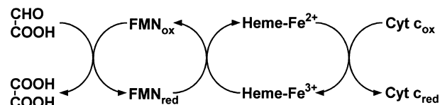
Fig. 4. A proposed scheme of electron-transferring function of the flavohemoprotein glyoxylate dehydrogenase during the oxidation of glyoxylate to form oxalate in the presence of cytochrome c .
